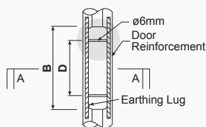
SERVICE DOOR DETAIL
