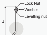
J-BOLT (6M-12M)
