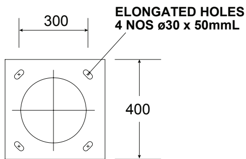
FLANGE PLATE
