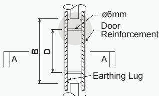
SERVICE DOOR DETAIL
