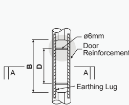
SERVICE DOOR DETAIL
