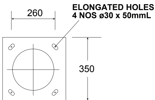
FLANGE PLATE 18 MM THICKNESS
