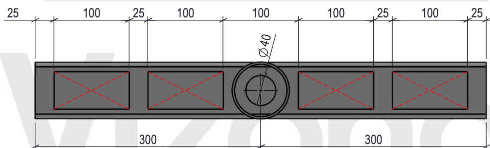
BOTTOM VIEW
