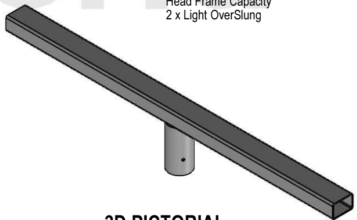
3D PICTORIAL
