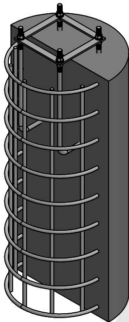
3D SECTION VIEW
