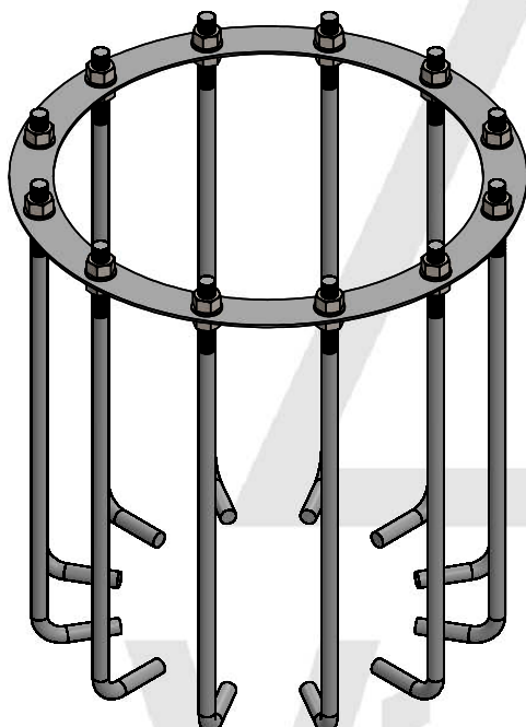
PICTORIAL VIEW
