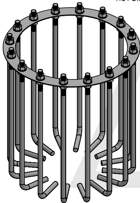
PICTORIAL VIEW
