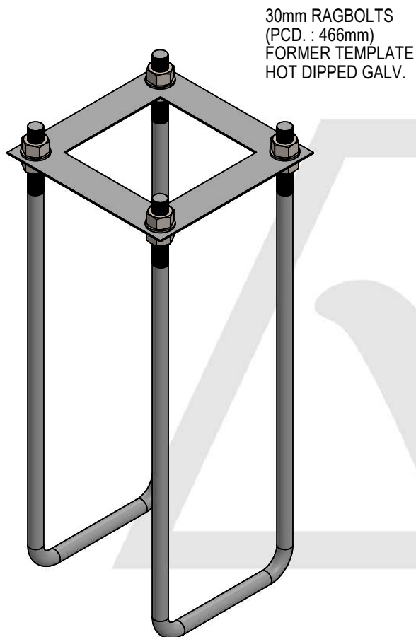
PICTORIAL VIEW
